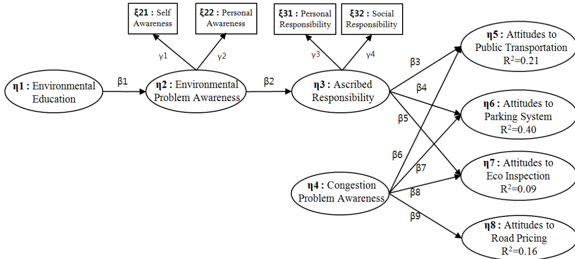
Figure 2. Estimated SEM (Civil Engineering Students Only, N=372)
